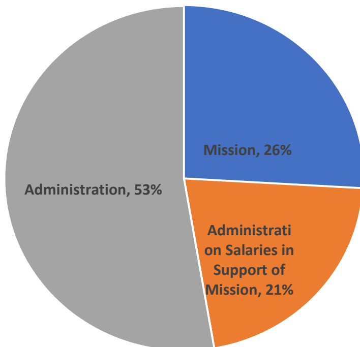
2018 DIOPA Budget
